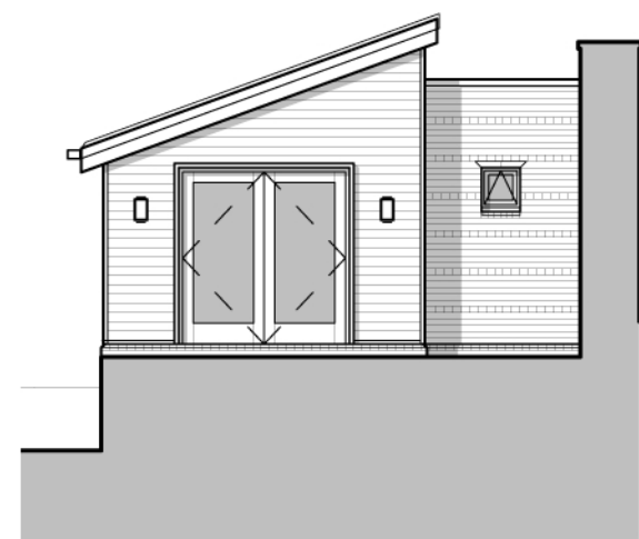
east elevation
