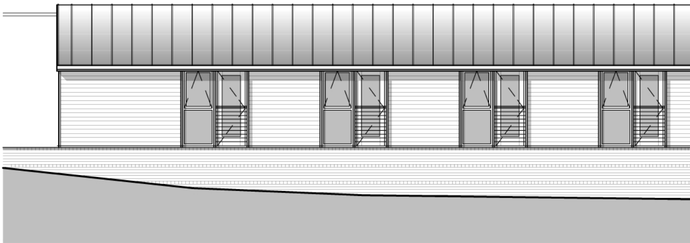
south elevation
